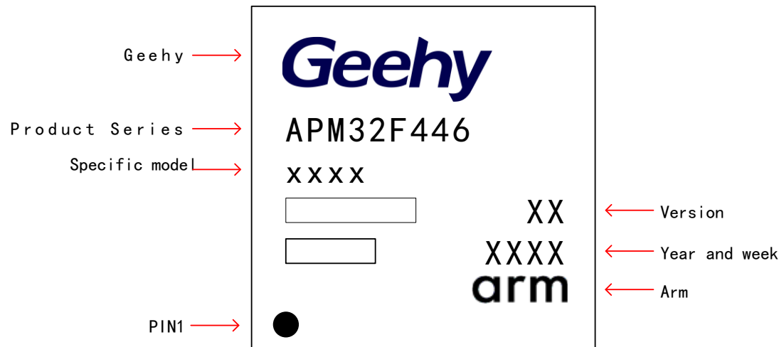
Figure 25 LQFP100 - 100 Pins, 14 x 14mm Diagram
